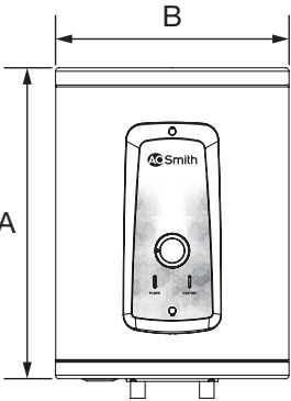
Front View All Dimensions in mm
